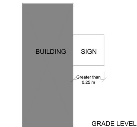
Figure 2-7: Illustration of Projecting Sign
