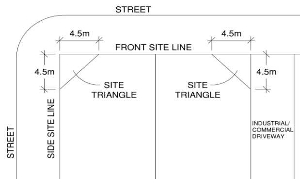
Figure 2-2: Sight Triangles
