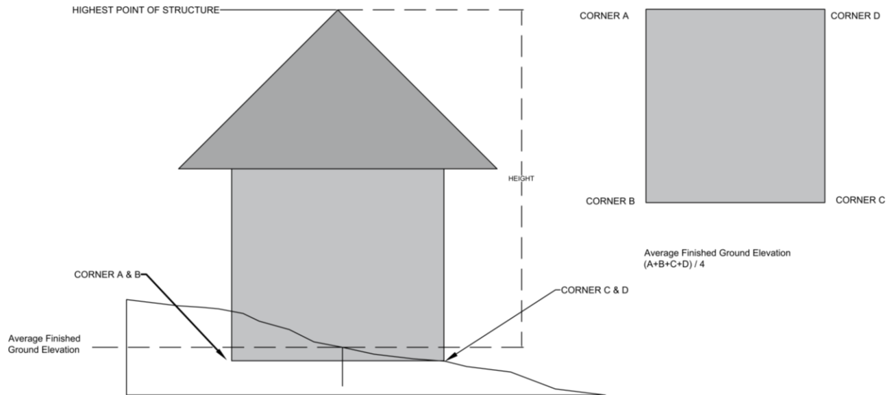
Figure 2-1: Building Height
