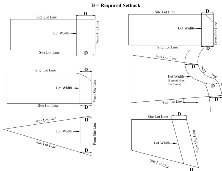
Figure 2-10: Illustrations of Site Width
